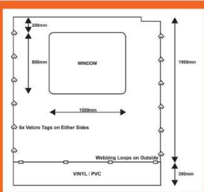
Technical Sketch
